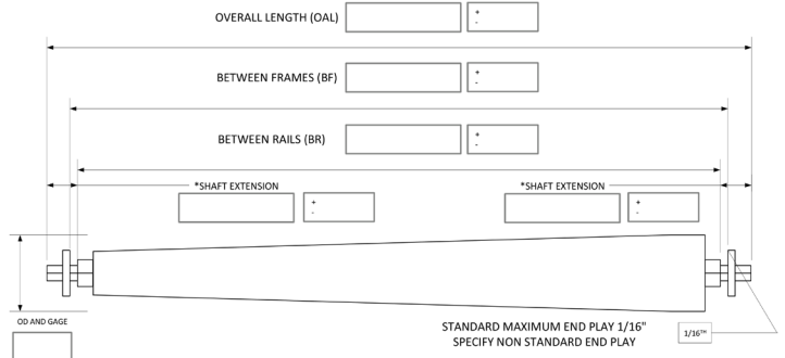
TAPERED ROLLER
