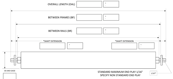
STRAIGHT ROLLER
