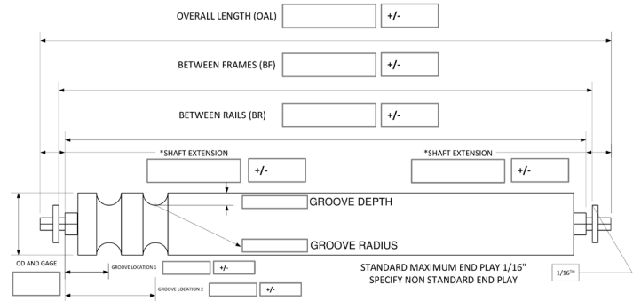
GROOVED ROLLER
