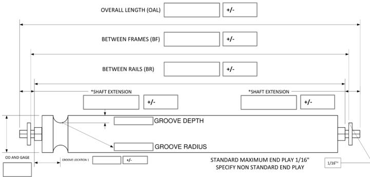
GROOVED ROLLER
