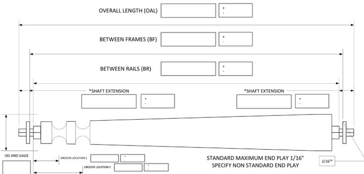
TAPERED ROLLER (GROOVED)
