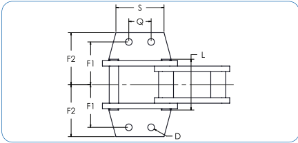
Dimensions (in)
