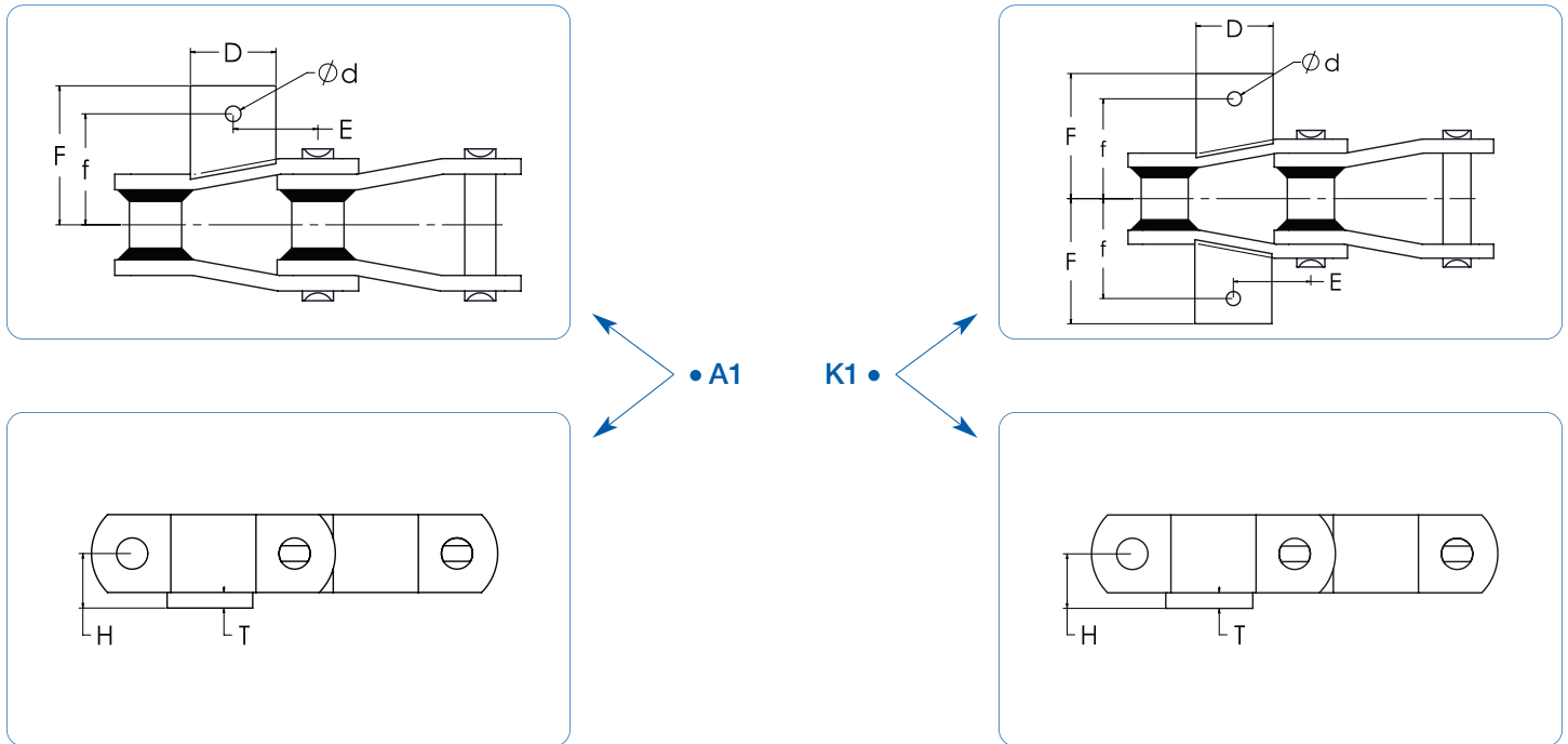
Dimensions (in)
