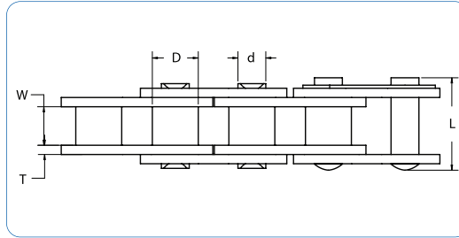
Dimensions (in)
