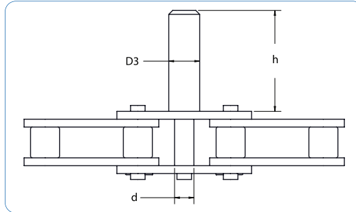
Dimensions (in)
